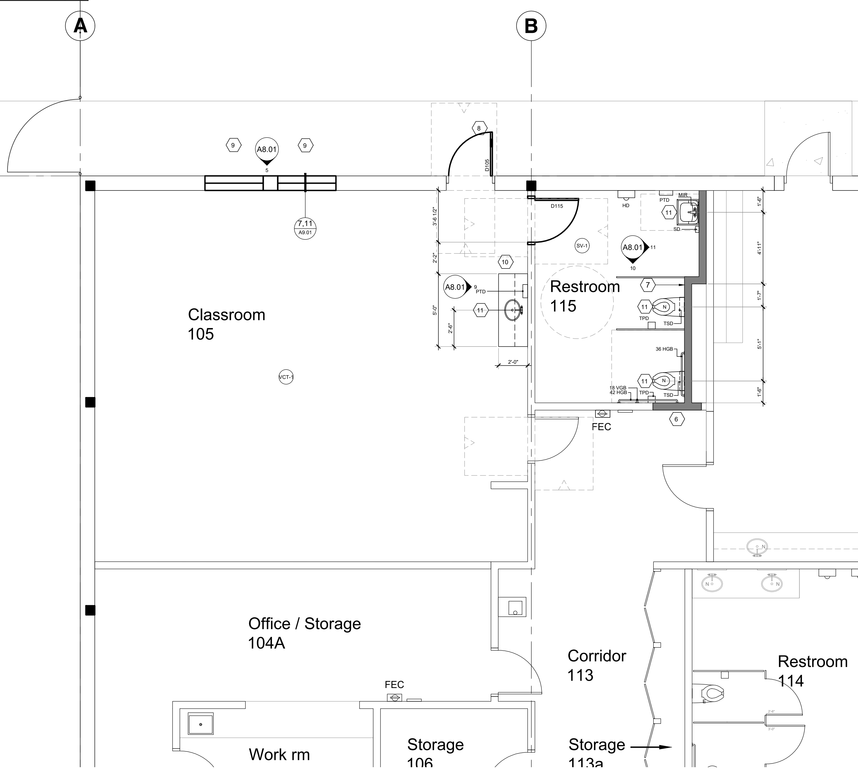
1 FLOOR PLAN A2.40 Scale 1/4"=1'-0"
