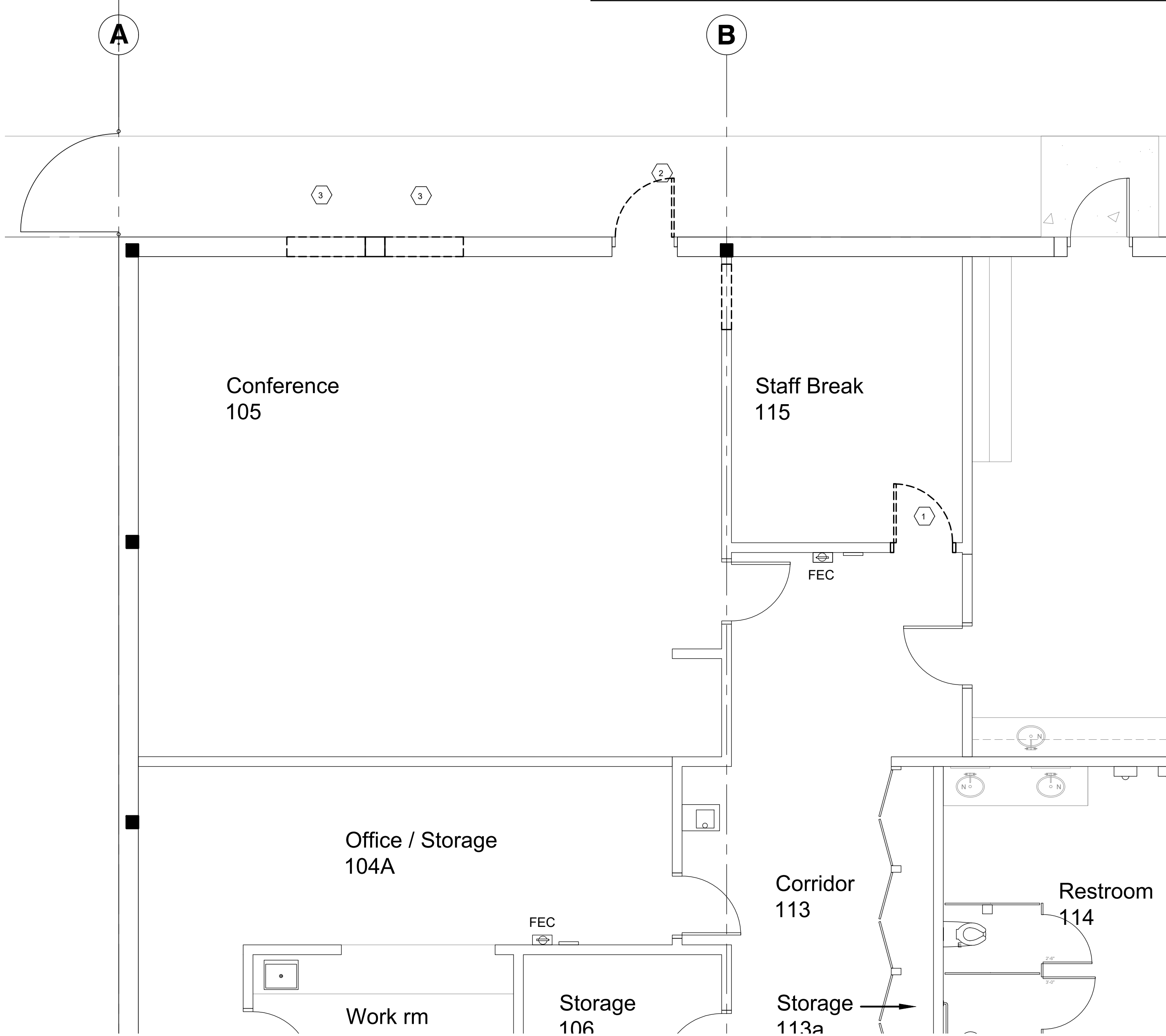
2 DEMO PLAN A2.40 Scale 1/4"=1'-0"
