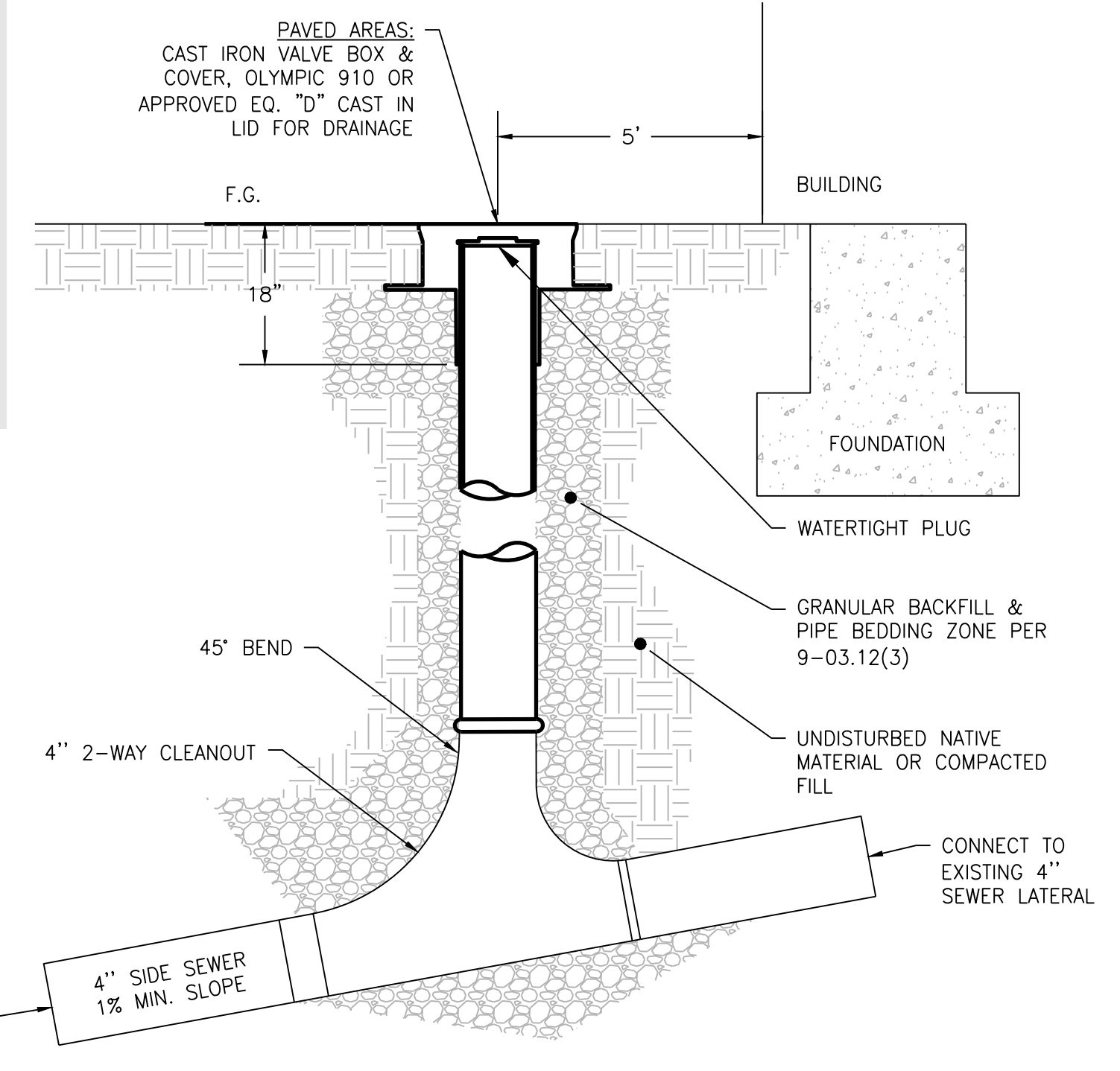
1 2-WAY SEWER CLEANOUT NO SCALE
