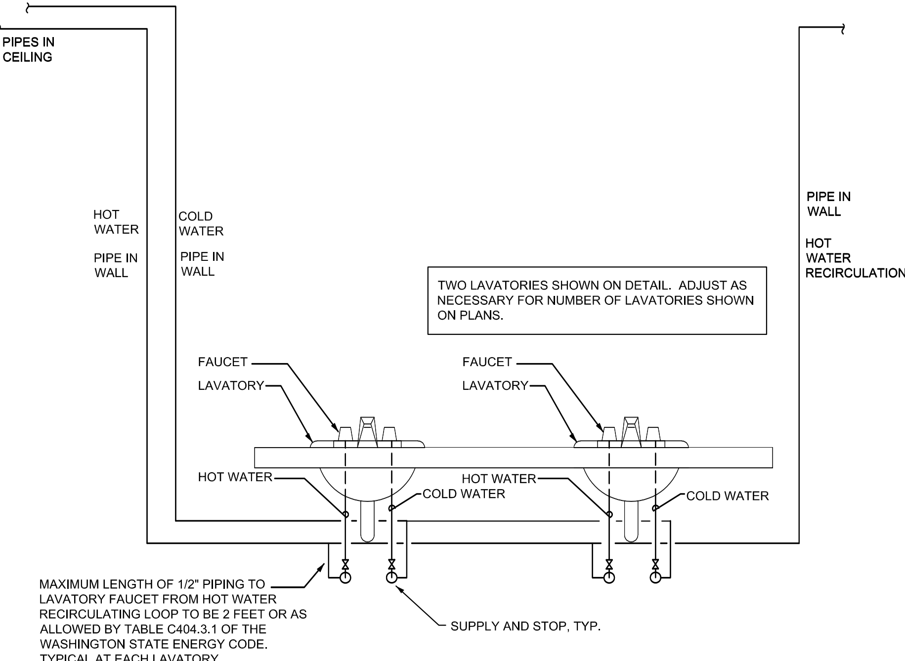
1 LAVATORY SUPPLY PIPING P3.00 DIAGRAMMATIC
