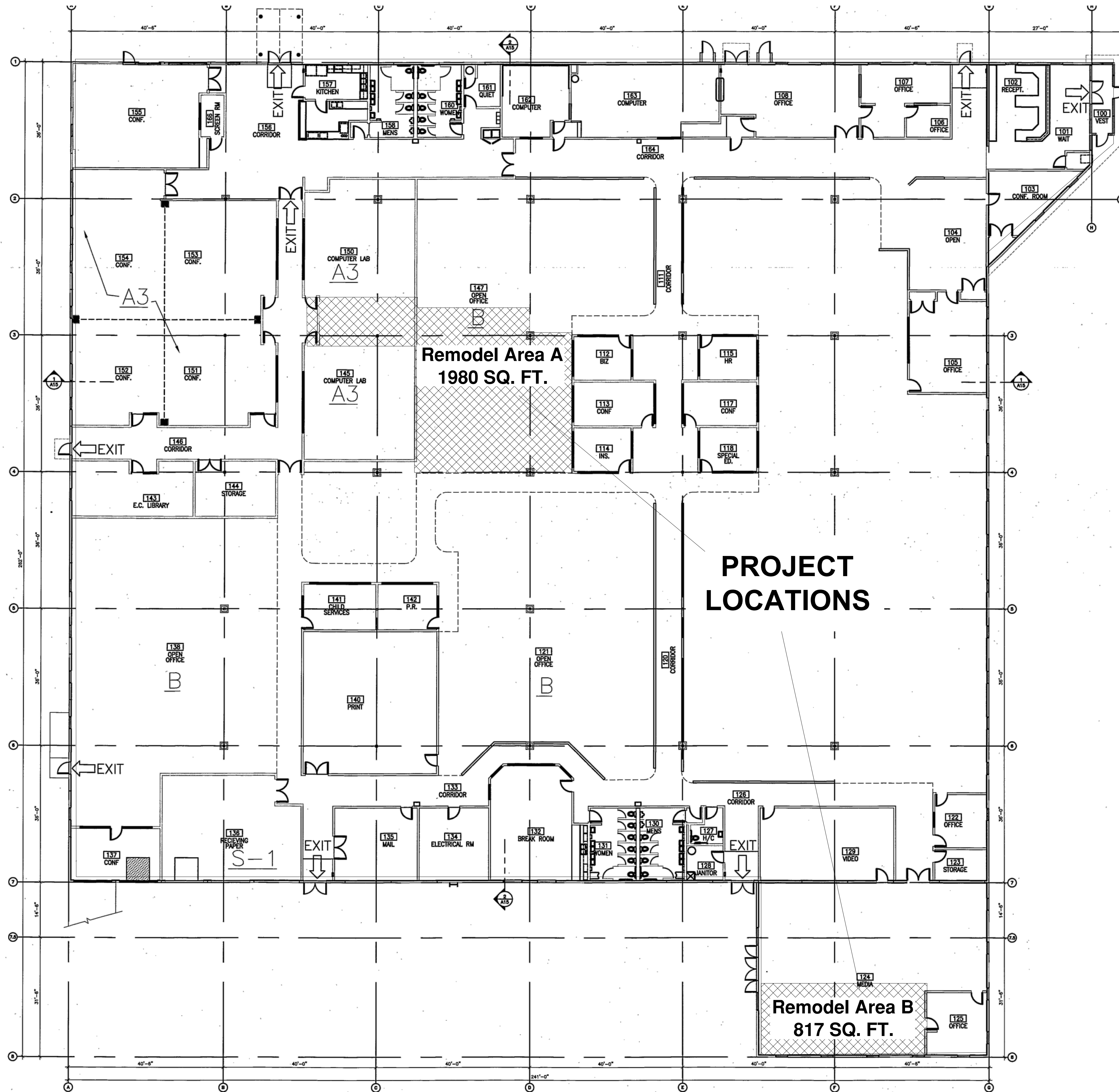
Project Location Plan - North Area A and South Area B scale: 3/8" = 1'-0"
